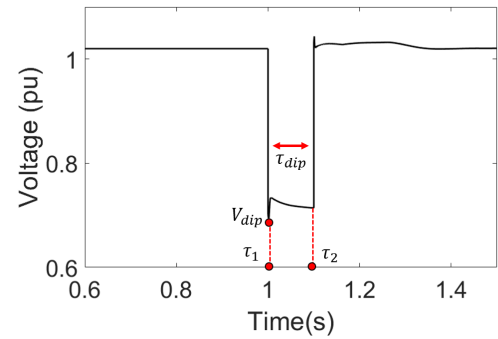
FIGURE 6. Transient stability index for S_\tau and S_v .
